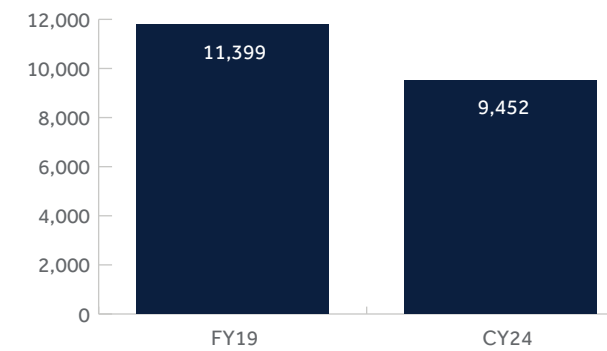
Scope 3 - Relevant Categories - All Manufacturing Locations (ktonnes CO 2 e)
