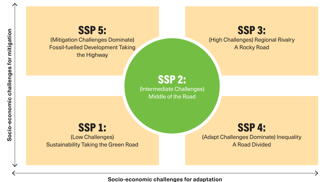
Fig. 1 Overview of SSPs (Narratives in O'Neill et al, 2016, Glob Env Change, online first)
