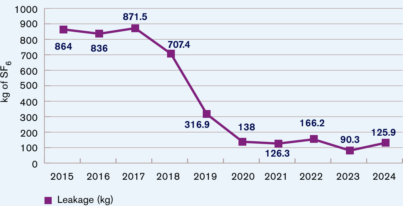
Figure 4 – SF6 gas leakage trends
