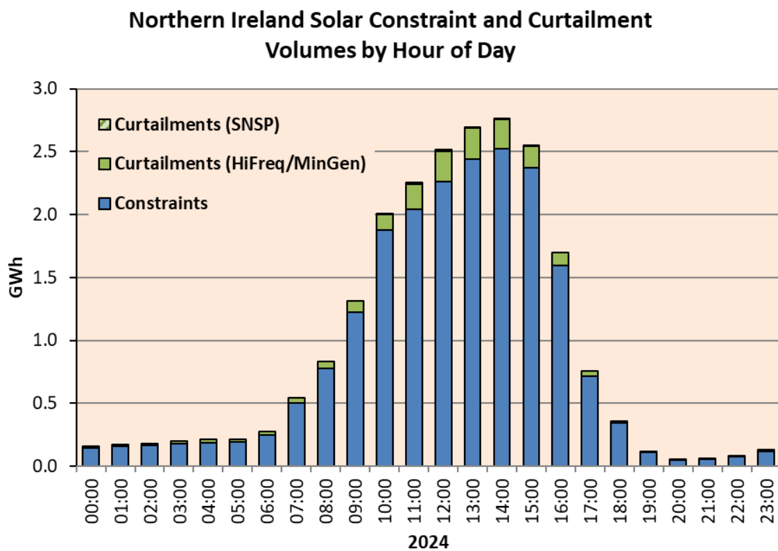
Figure 24: Breakdown of solar constraints and curtailments in NI in 2024 by hour of day
