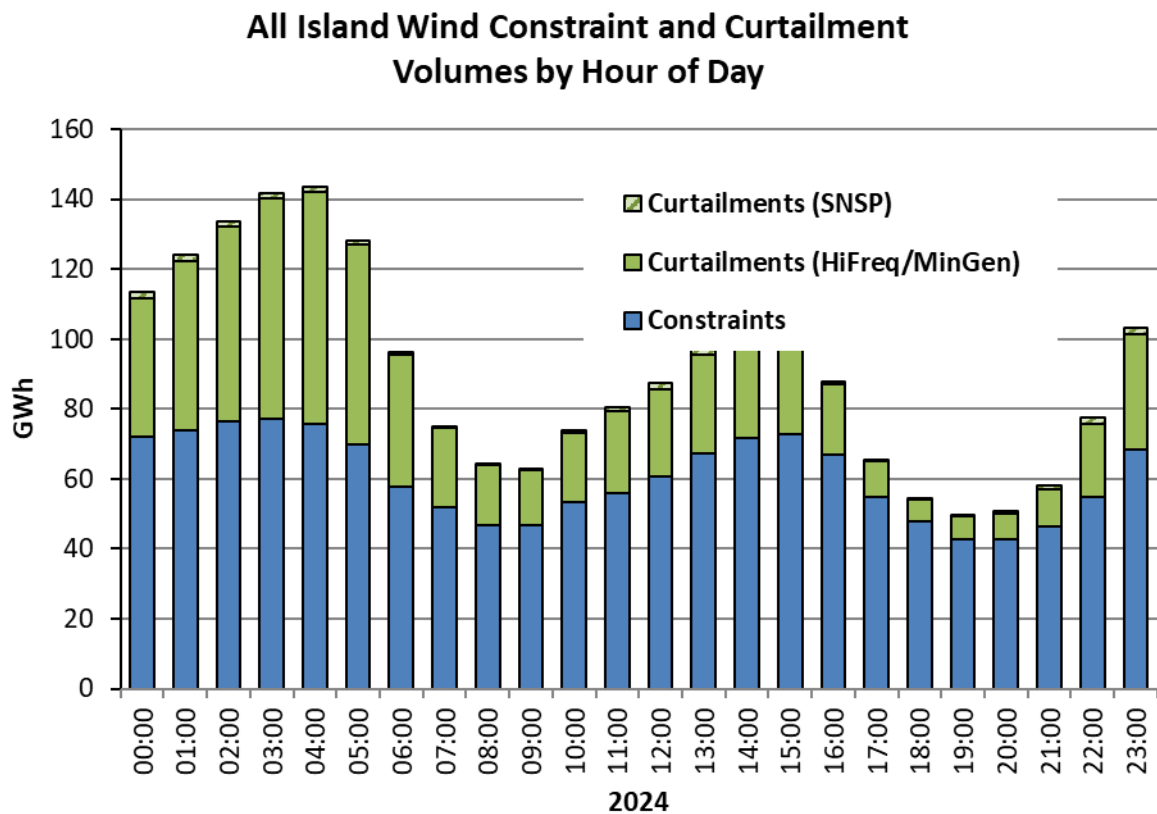
Figure 19: All-Island breakdown of wind constraints and curtailments in 2024 by hour of day
