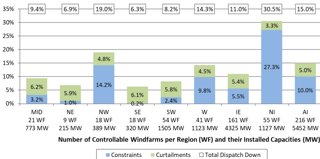
Figure 6: Regional/Jurisdictional Controllable Wind Dispatch-Down Percentages in 2024
