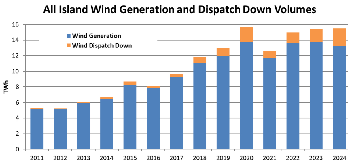
Figure 1: All Island Annual Wind Generation and Dispatch Down Volumes
