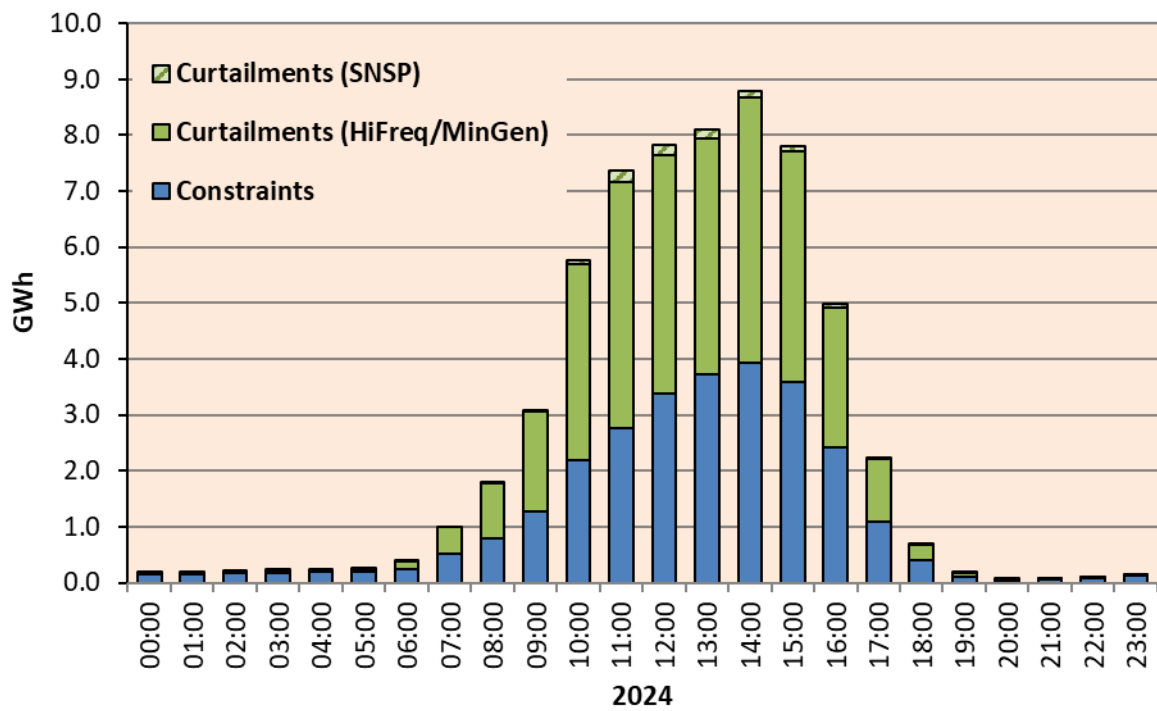
Figure 22: All-Island breakdown of solar constraints and curtailments in 2024 by hour of day
