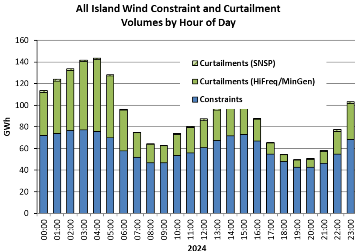
Figure 5: All-Island breakdown of wind constraints and curtailments in 2024 by hour of day
