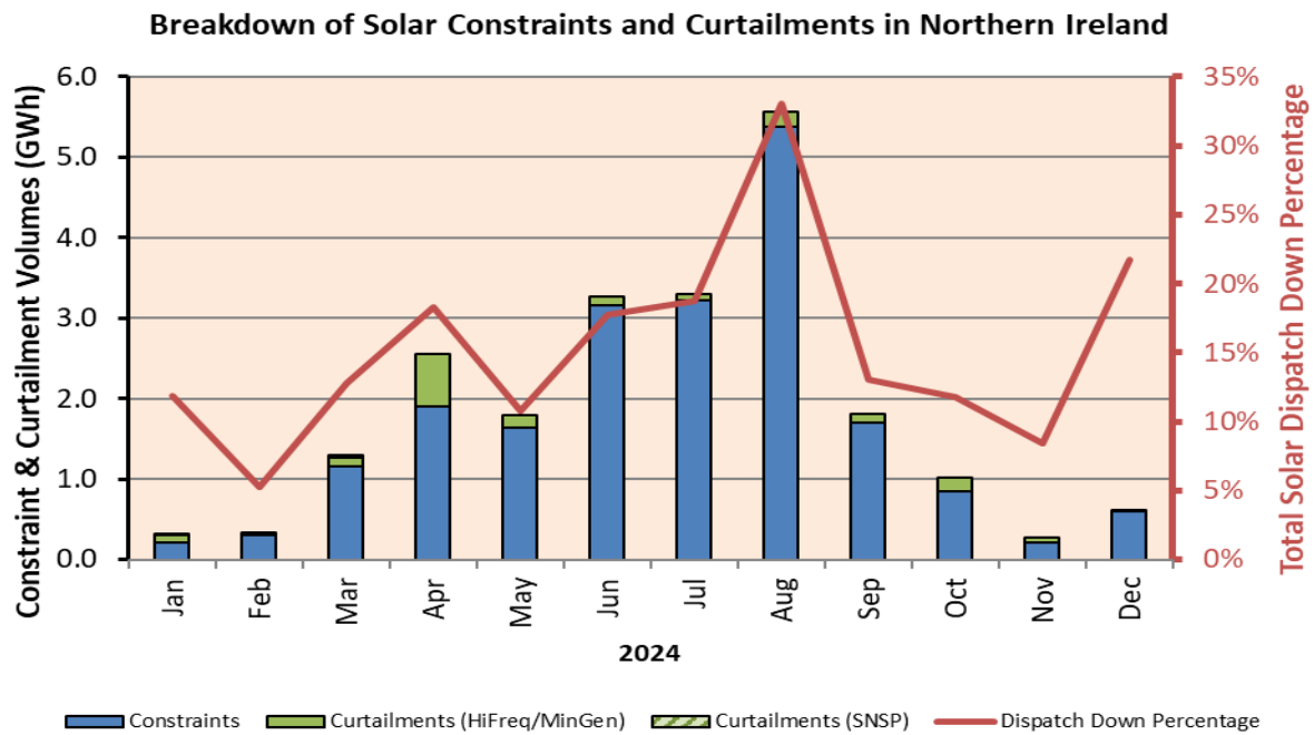
Figure 17: Monthly breakdown of solar dispatch-down categories in Northern Ireland in 2024
