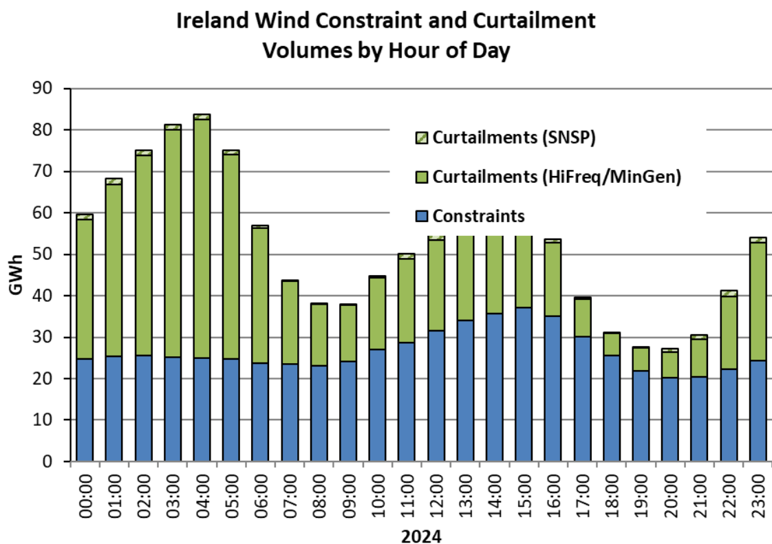
Figure 20: Breakdown of wind constraints and curtailments In Ireland in 2024 by hour of day
