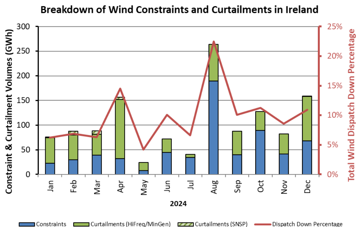
Figure 9: Monthly breakdown of the main wind dispatch-down categories in Ireland in 2024
