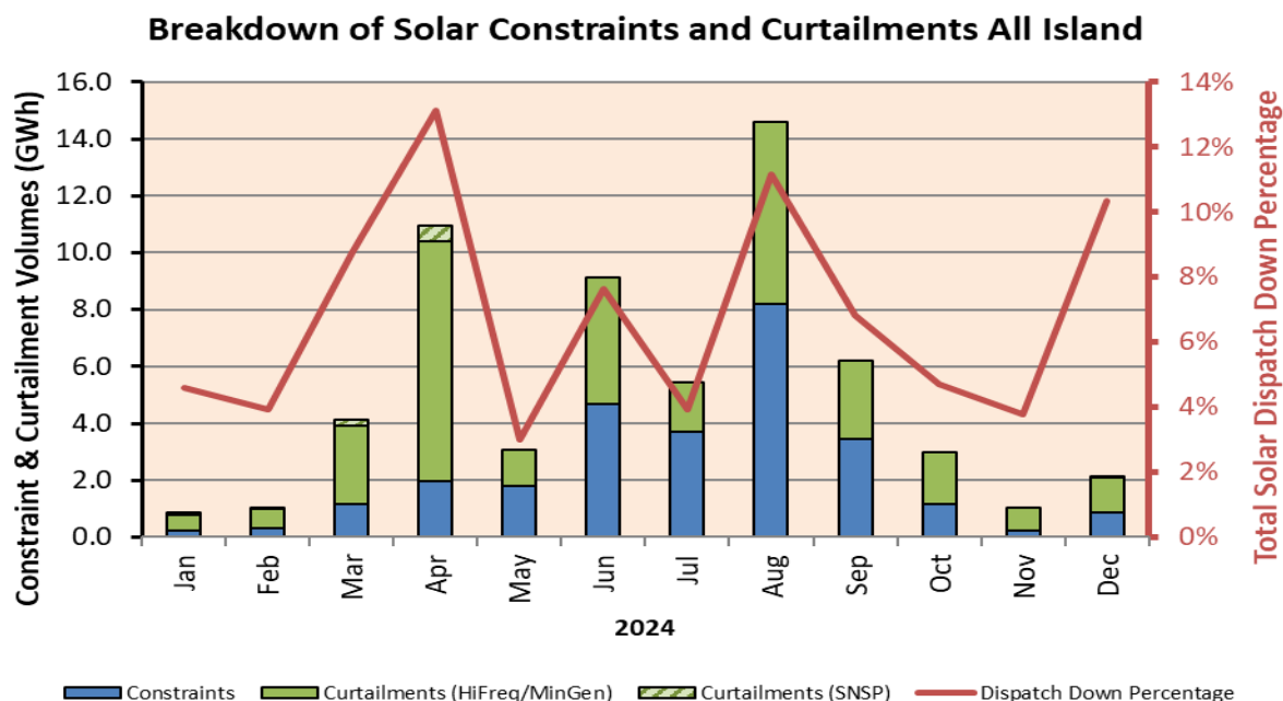
Figure 13: Monthly breakdown of all-island solar constraints and curtailments in 2024
