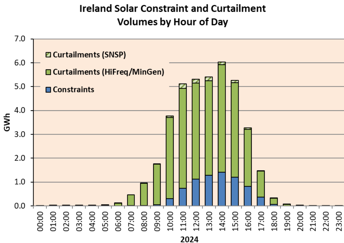
Figure 23: Breakdown of solar constraints and curtailments In Ireland in 2024 by hour of day
