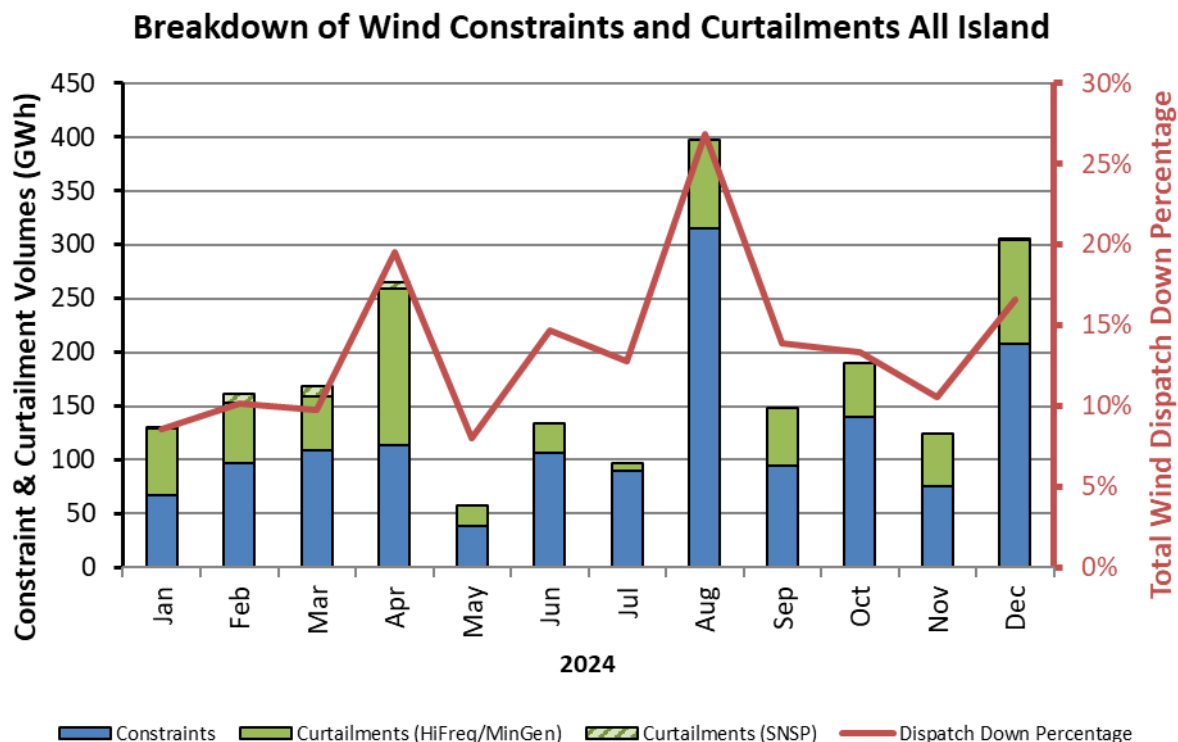
Figure 7: Monthly breakdown of all-island wind constraints and curtailments in 2024
