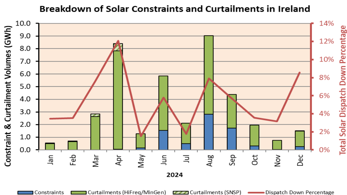
Figure 15: Monthly breakdown of the main solar dispatch-down categories in Ireland in 2024
