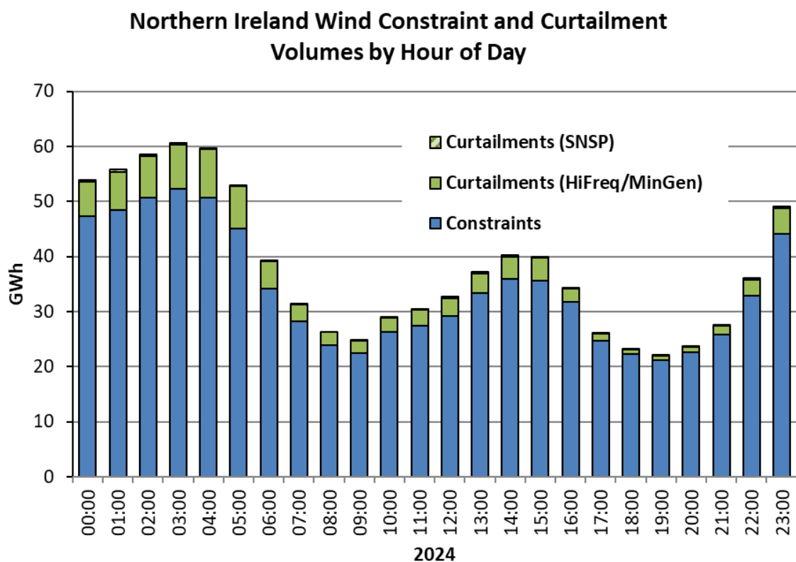
Figure 21: Breakdown of wind constraints and curtailments in NI in 2024 by hour of day
