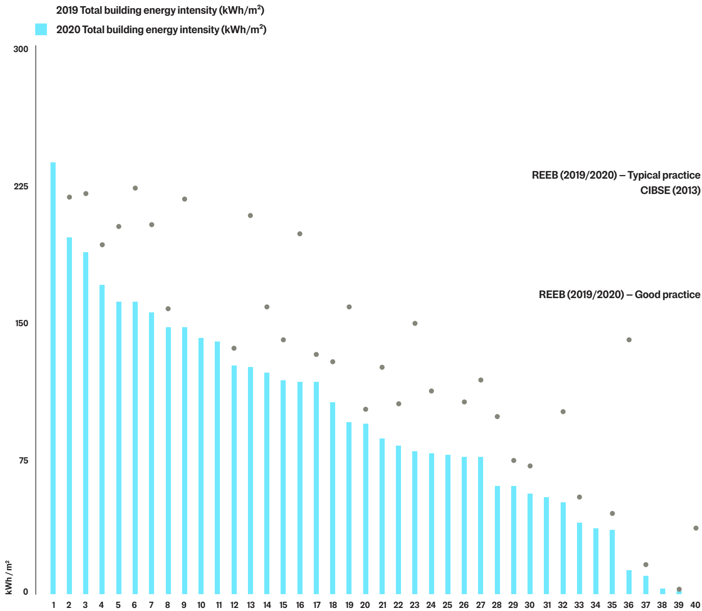
Total building energy performance (landlord and tenant) (kWh/m 2 )
