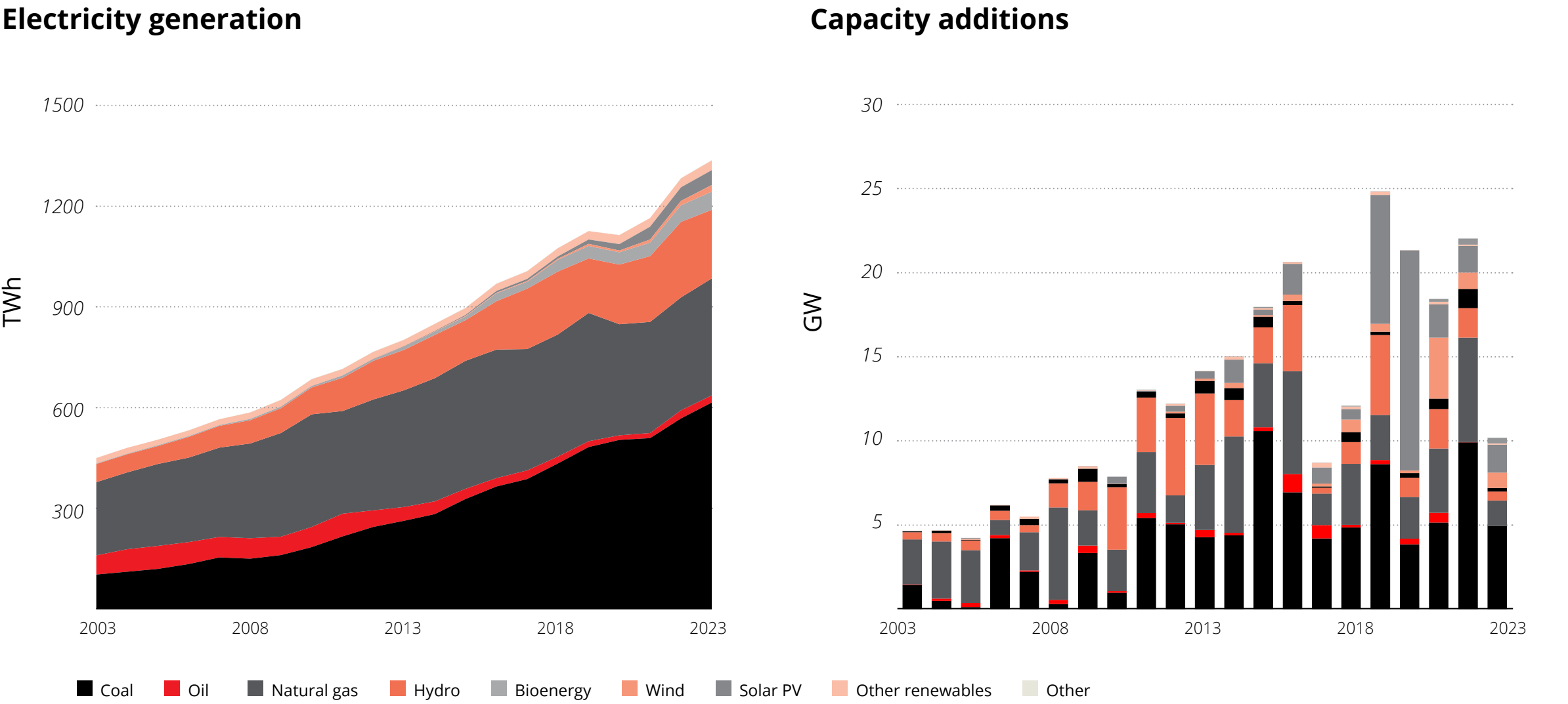
Figure 2. Southeast Asia electricity generation and annual electricity generation capacity additions by source, 2003-2023
