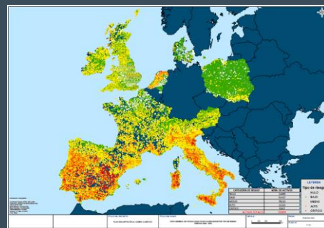
Period 2041-2070
