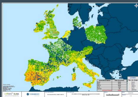
Current Period-2040
