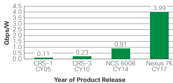
Figure 26. System Performance Improvements, Gbps/W
