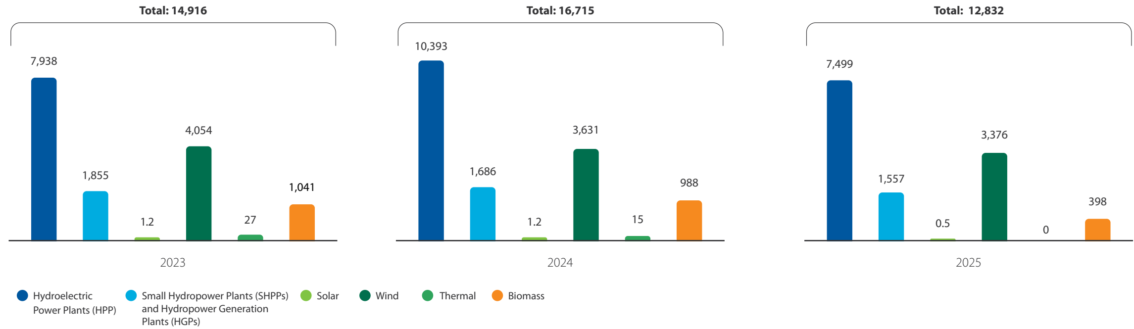
Net Energy Production by Source (GWh) GRI EU-02
