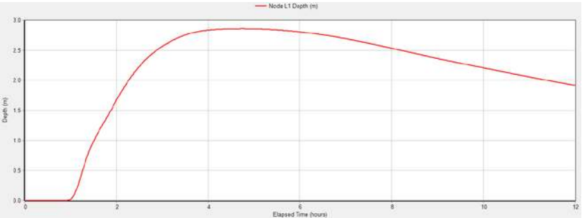
Figure 2: Level reached in lamination space I for 81 mm rain.
