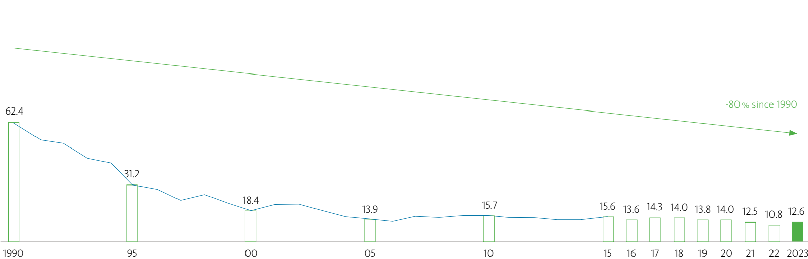
Fig. 2.5: Copper emissions at the Hamburg site Copper in g/t of copper output
