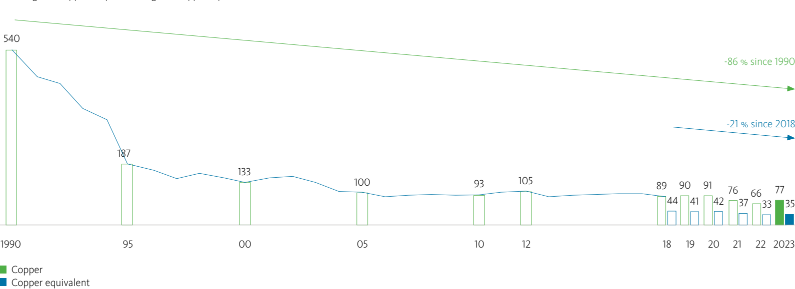
Fig. 2.4: Dust emissions at the Hamburg site Dust in g/t of copper output and in g/t of copper equivalent
