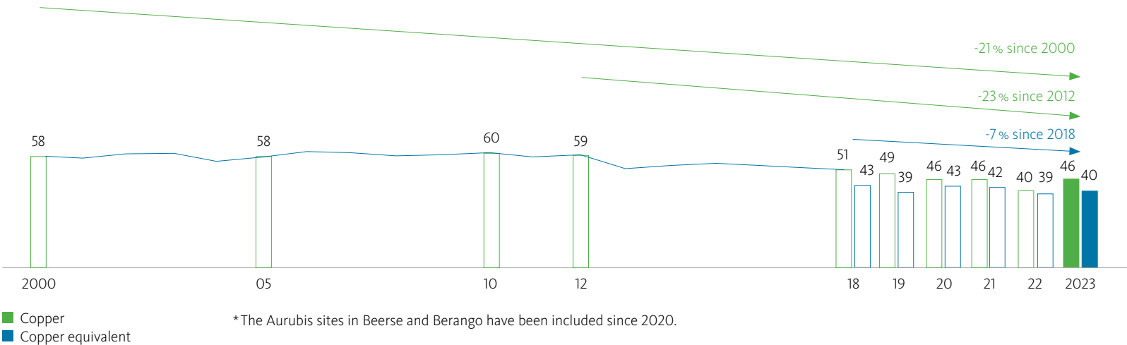
Fig. 1.17: Water withdrawal in Aurubis Group copper production* Water withdrawal in m³/t of copper output
