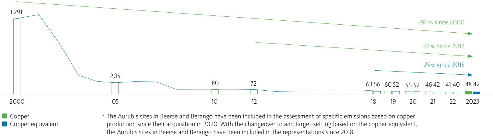
Fig. 1.15: Successful reduction of dust emissions in Aurubis Group copper/multimetal production* Dust emissions in g/t of copper output and in g/t of copper equivalent
