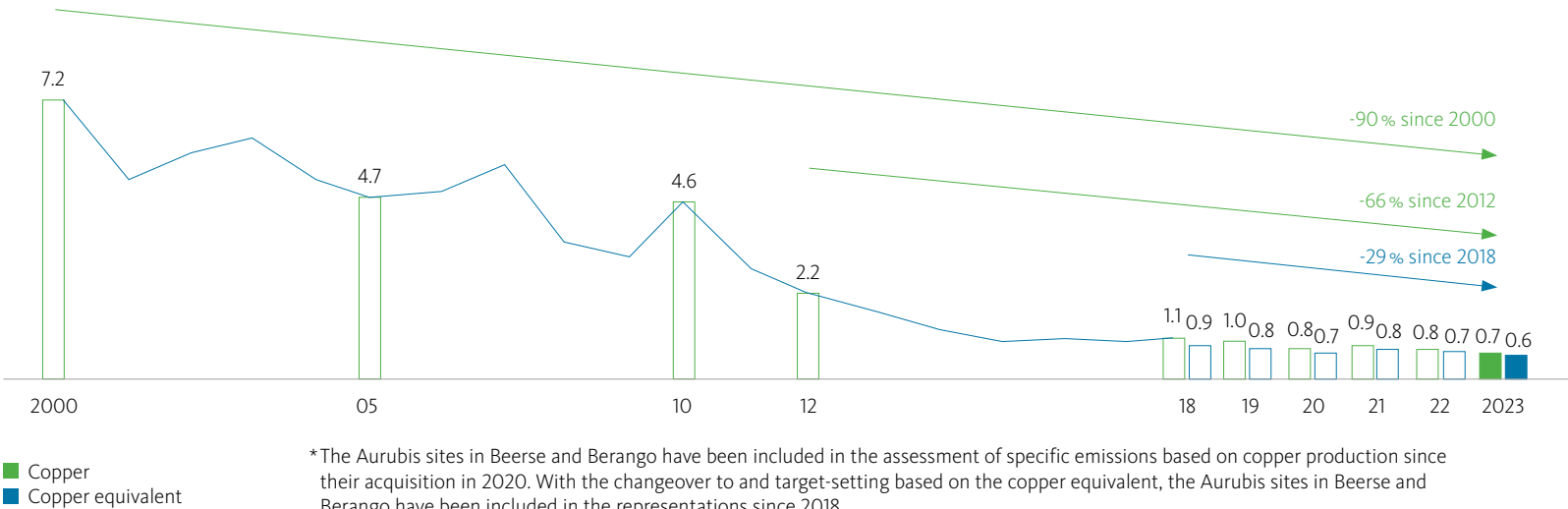
Fig. 1.18: Metal emissions¹ to water in Aurubis Group copper/multimetal production* Metal emissions to water in g/t of copper output and in g/t of copper equivalent
