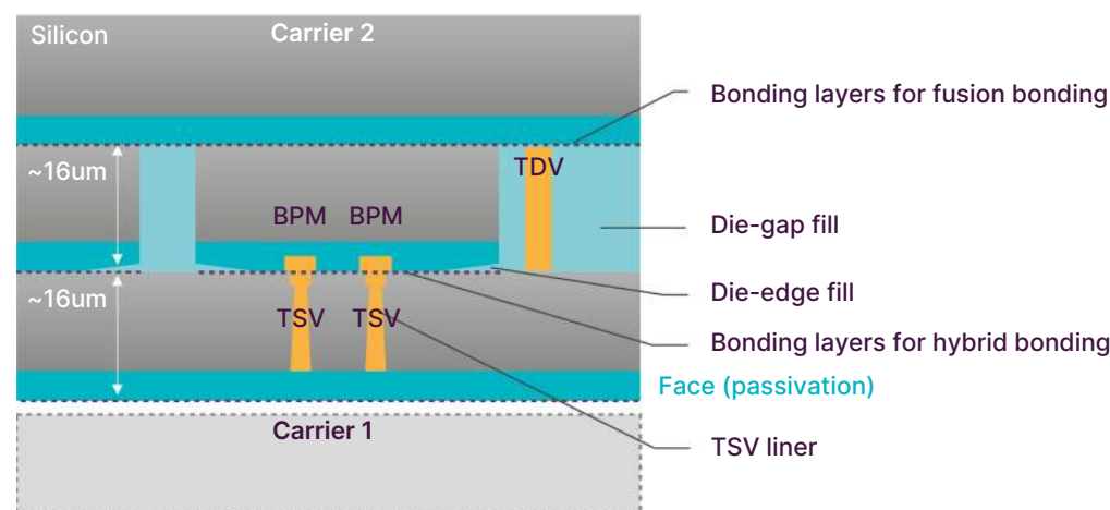
AP applications example: SoIC (Systems on IC)
