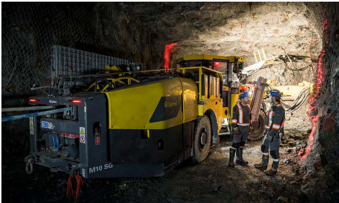
Battery electric bolter at Odyssey (Quebec, Canada).
